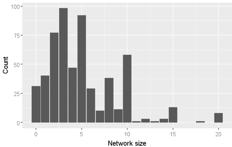
Figure 6: Histogram of network size (unweighted)
